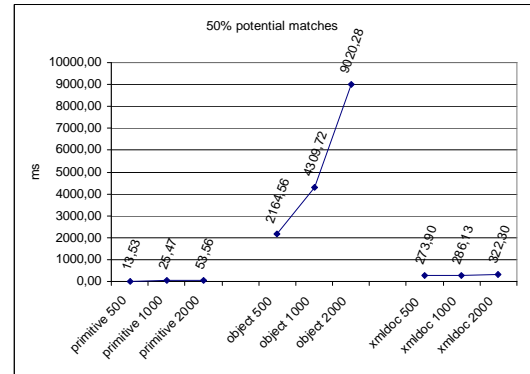
(b) 50% potential matches
