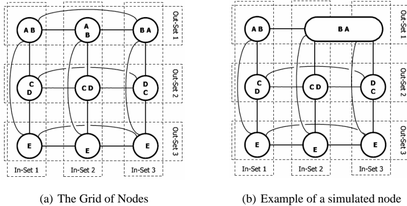
Figure 2: Intermediate Replication of Tupespaces
